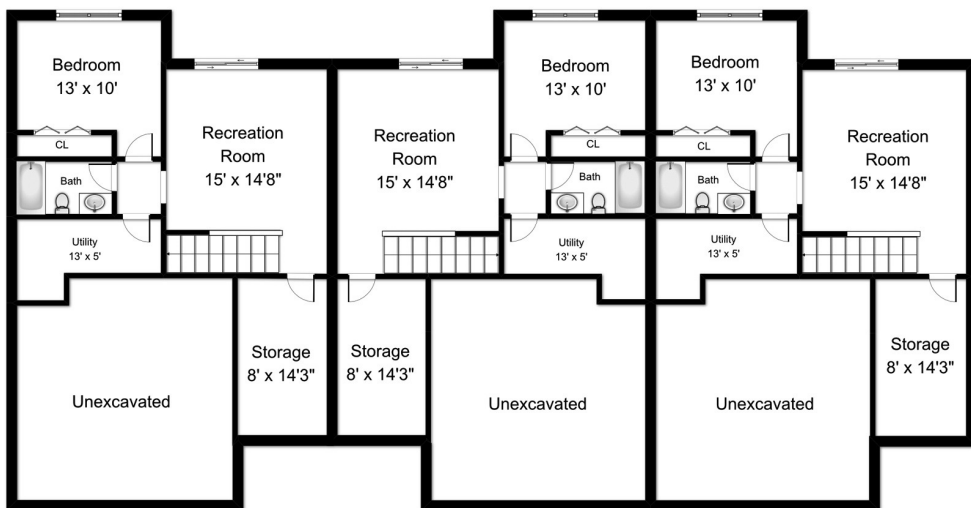
Lower Level
