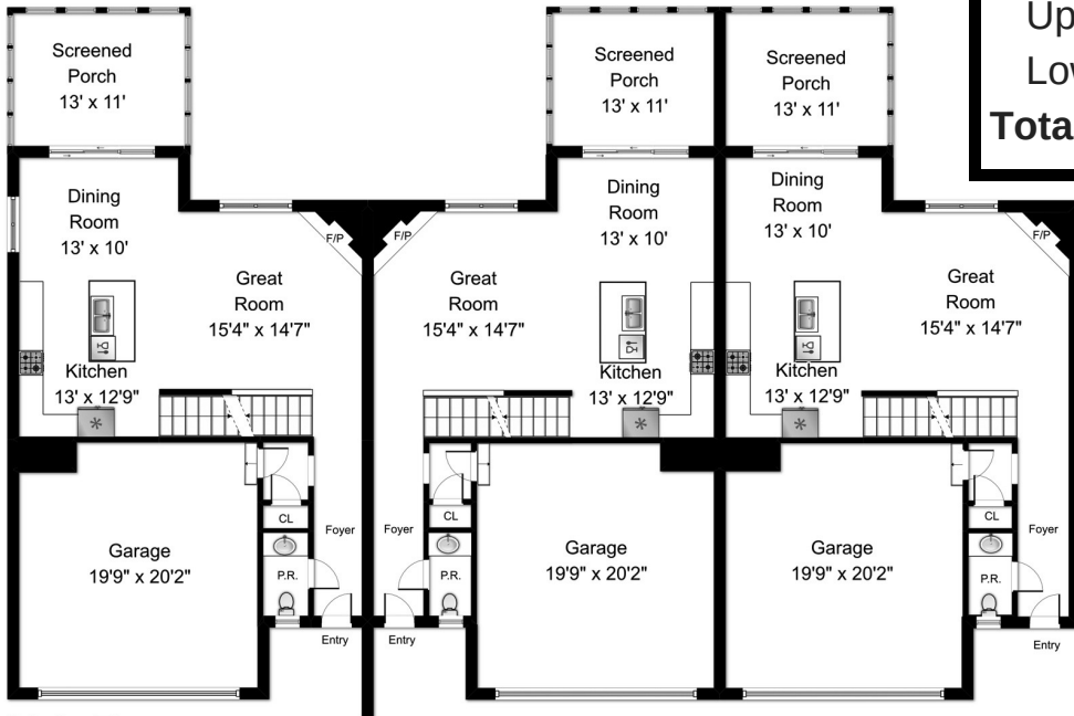
Main Floor
